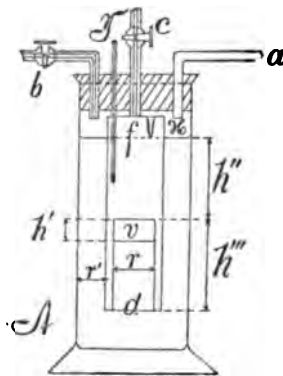
FIG. 4.—Cartesian diver with double tube.
